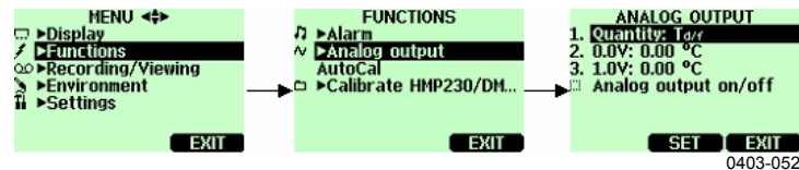
Figure 8 Analog Output
