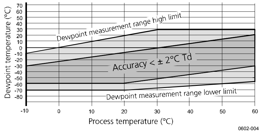
Figure 32 DMP74B Accuracy
