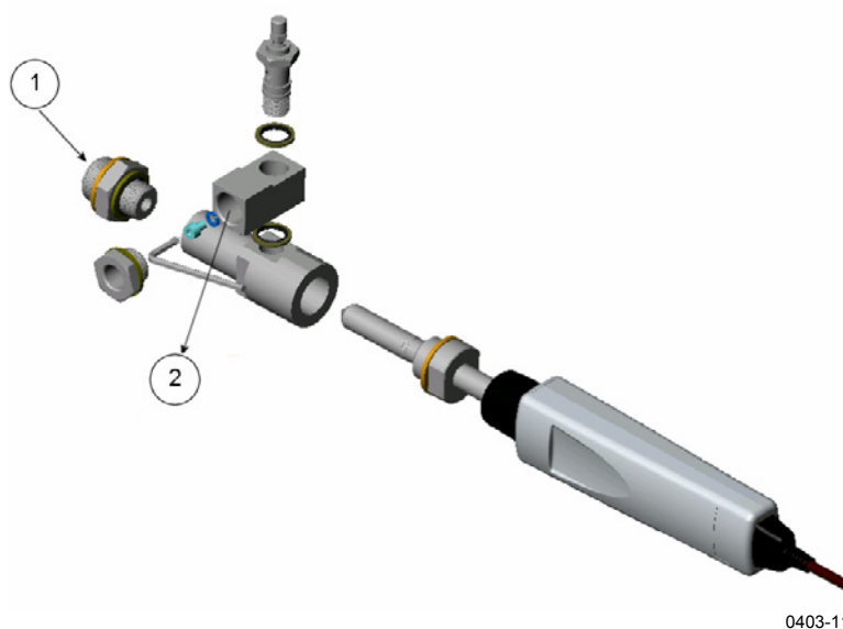
Figure 21 DSC74B
