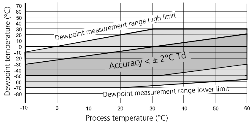
Figure 33 DMP74C Accuracy
