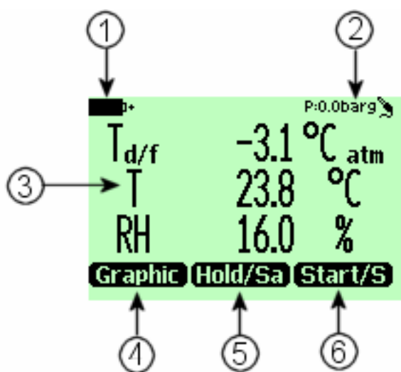
Figure 4 Basic Display
