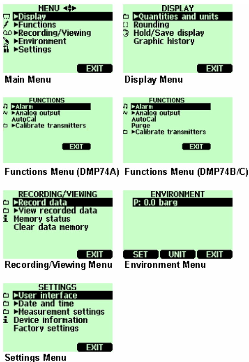
Figure 5 Menus
