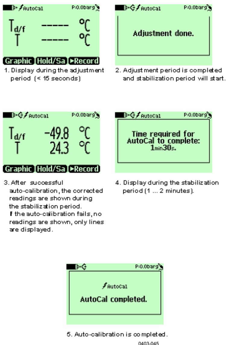
Figure 9 Auto-Calibration Displays
