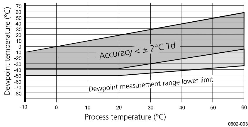
Figure 31 DMP74A Accuracy
